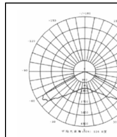
Light Distribution Curve
